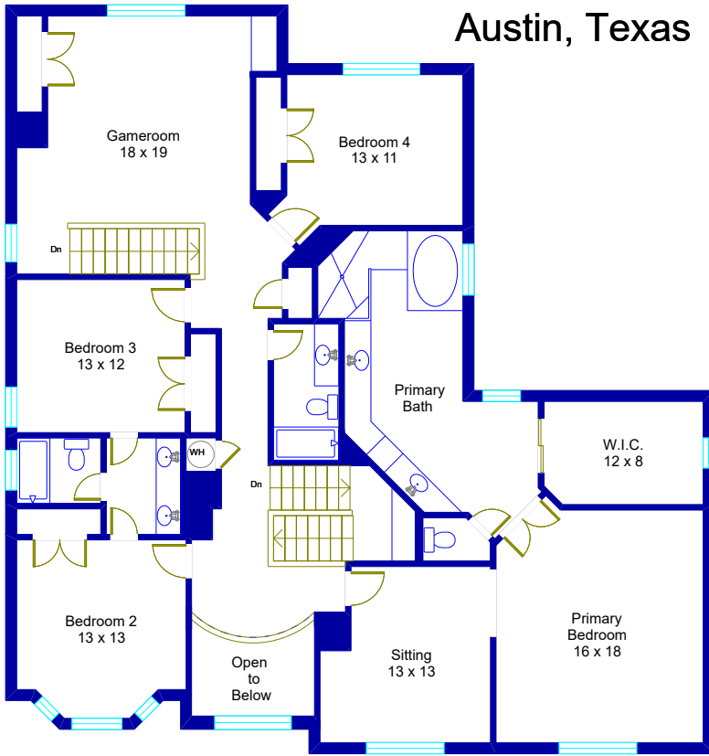
Main House Second Floor
